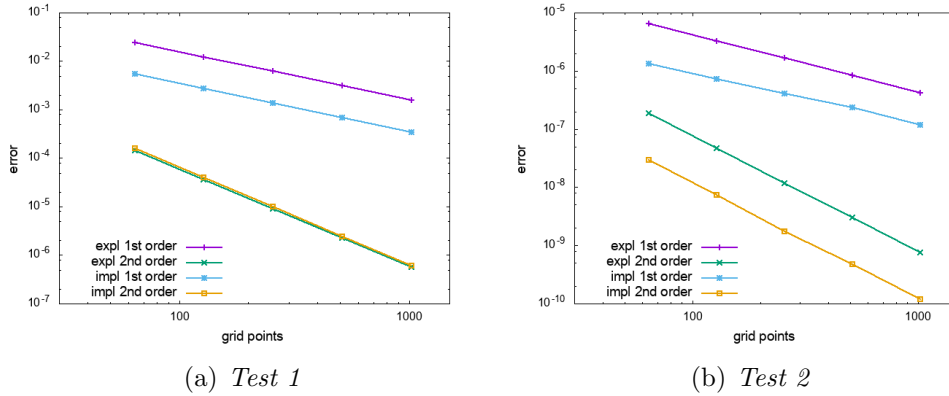
Figure 4: Perfect gas nozzle flow: L_\infty numerical error on pressure. Left panel: gas nozzle flow test 1 . Right panel: gas nozzle flow test 2 .
