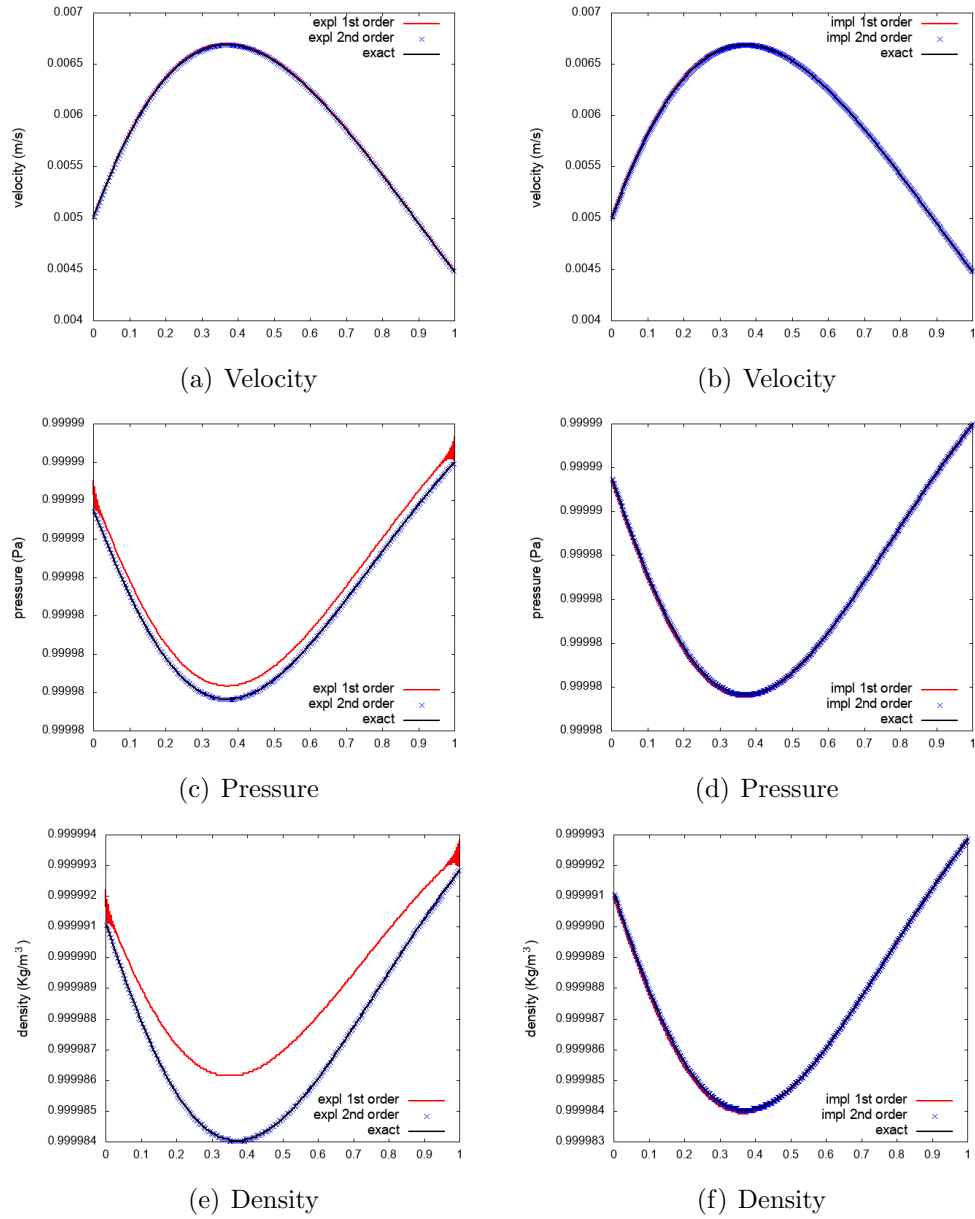
Figure 3: Perfect gas nozzle flow test 2 : velocity, pressure and density. Left column: explicit relaxation scheme. Right column: implicit relaxation scheme.
