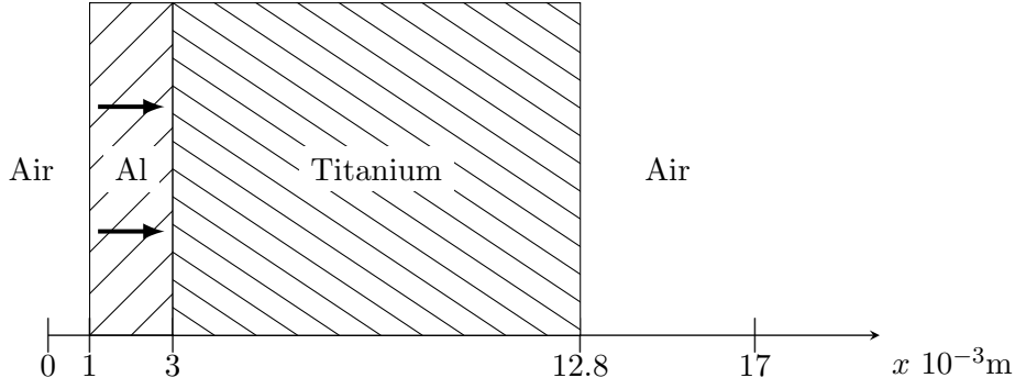
Fig. 4. Sketch of the initial configuration for TC1
