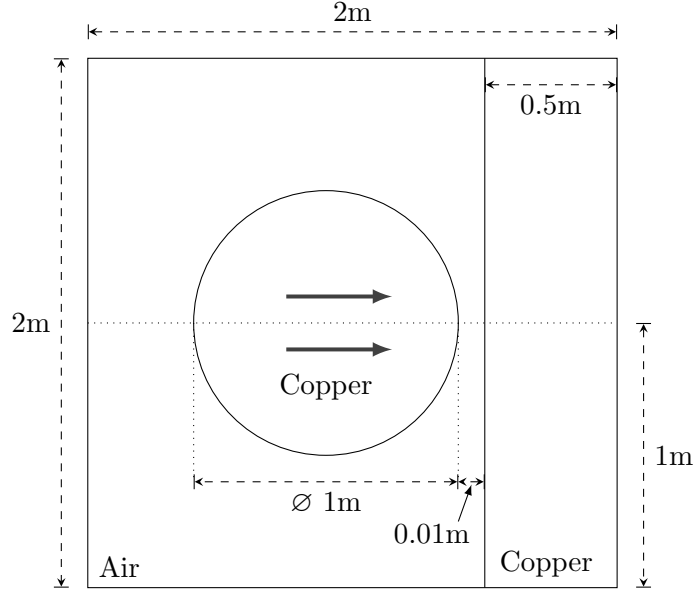
Fig. 9. Sketch of the initial configuration for TC3
