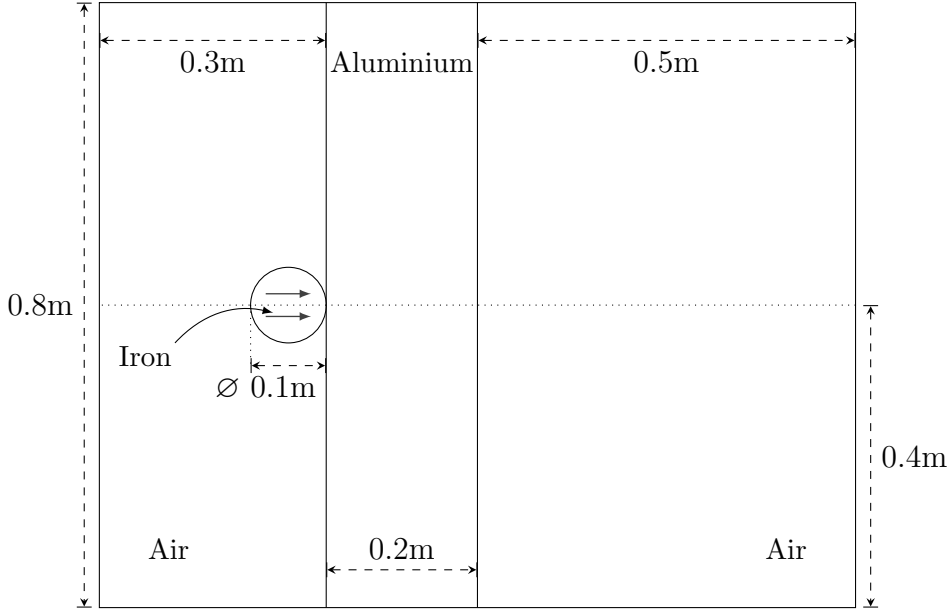
Fig. 7. Sketch of the initial configuration for TC2
