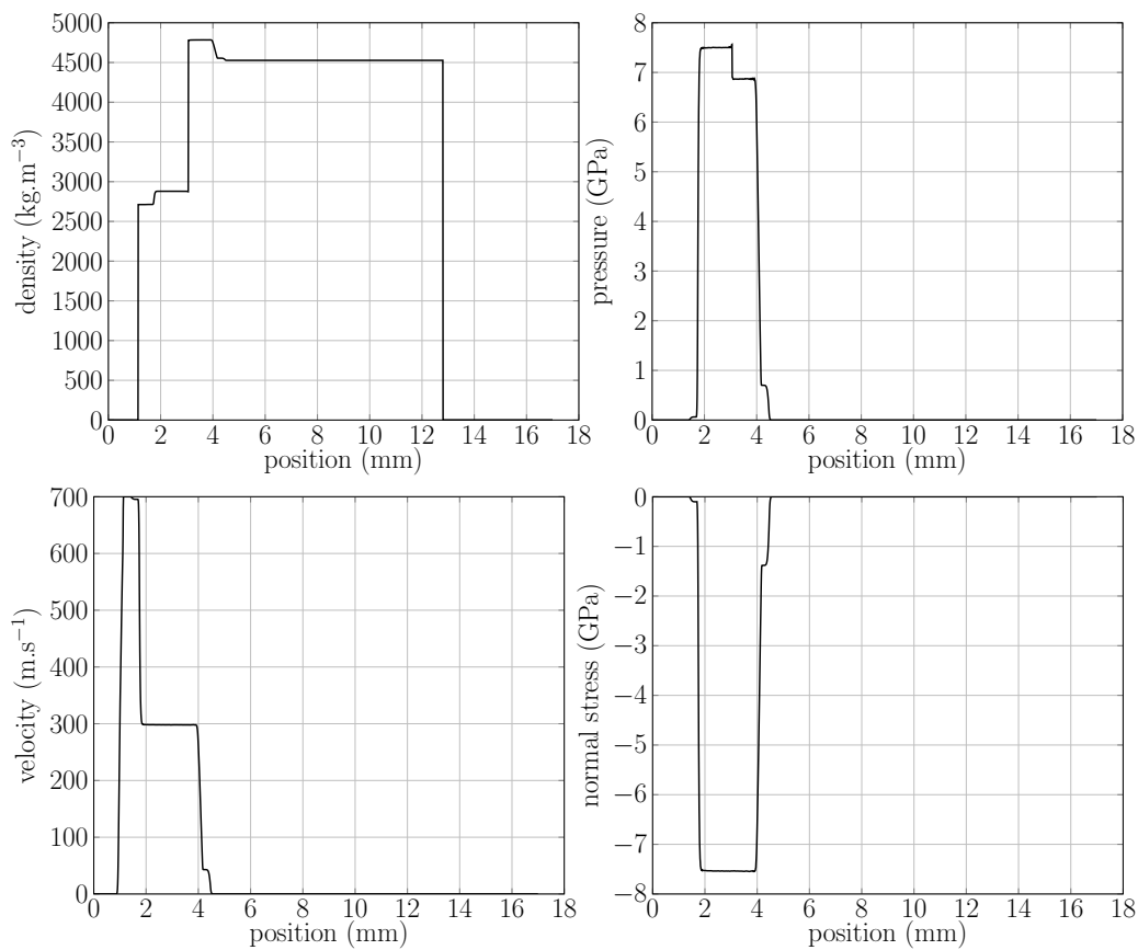
Fig. 6. TC1: Solution at t = 0.2\mu\text{s} for density, pressure, velocity and normal stress
