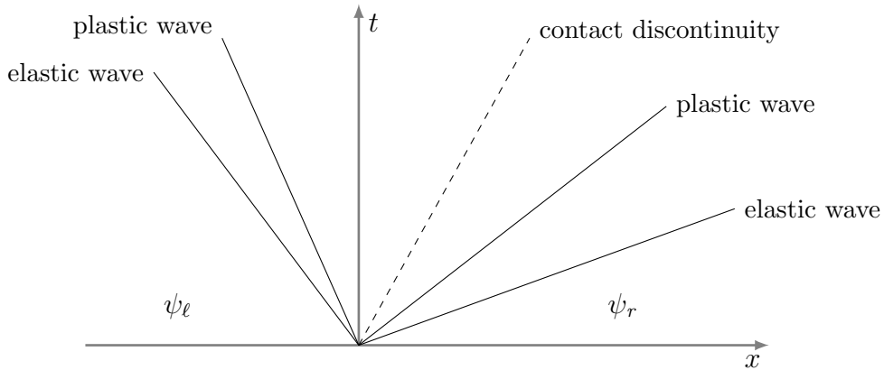
Fig. 5. Solution pattern of elasto-plastic problem.
