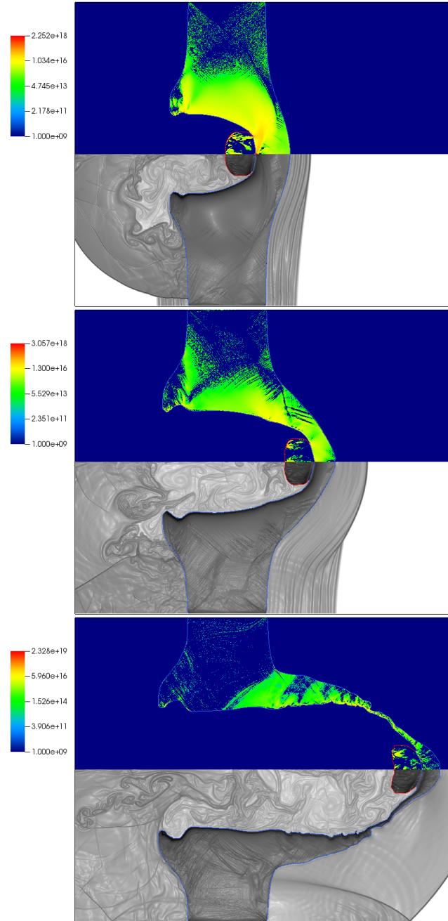
Fig. 8. TC2: Impact of iron on aluminium. Schlieren image and von Mises criteria at t = 0.03\text{ms} , 0.06\text{ms} , 0.13\text{ms} , 0.26\text{ms} , 0.53\text{ms} and t = 1.04\text{ms} .
