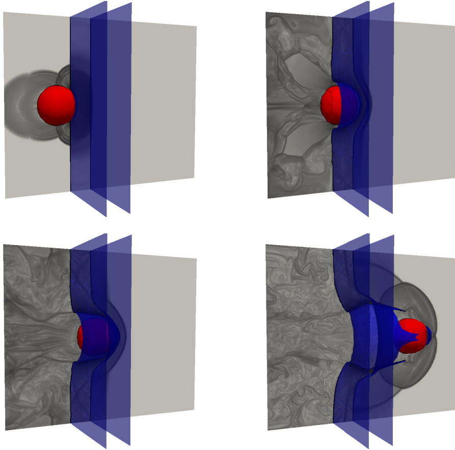
Fig. 12. TC4: Impact of Iron on Aluminium. Interfaces and Schlieren image at t = 110\mu s, 227\mu s, 337\mu s and 675\mu s from left to right, top to bottom
