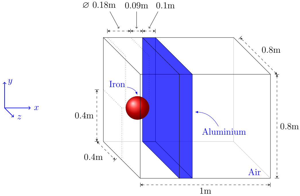
Fig. 11. Sketch of the initial configuration for TC4
