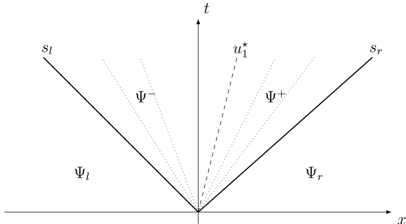
Fig. 2. HLLC solver wave pattern.
