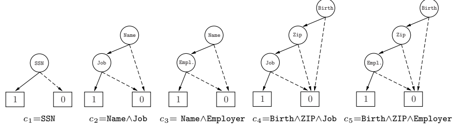
Fig. 4. OBDDs representing the confidentiality constraints in Figure 3
