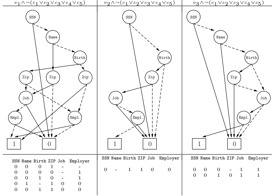
Fig. 7. OBDDs representing the composition of each visibility constraint in Figure 5 with the negated disjunction of the confidentiality constraints in Figure 4, and their one-paths
