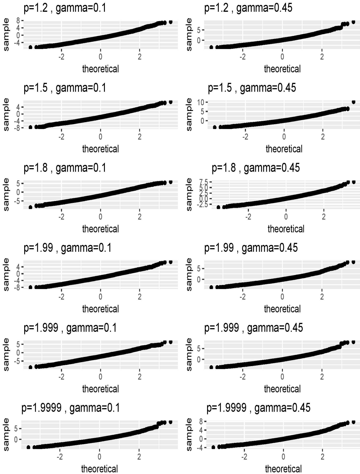
Figure 8: As before with scatters for \widehat{W}_{\hat{\tau}_n(p, \alpha_n; 2)} .
