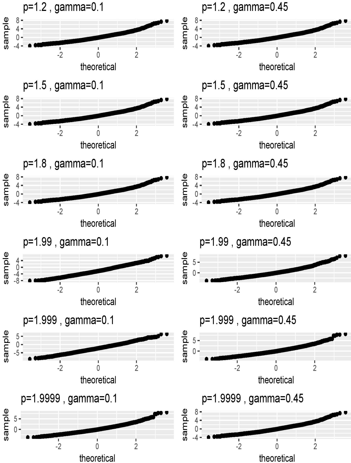
Figure 7: Q-Q -plots on quality of asymptotic approximations. Each plot shows the sample quantiles of \widetilde{W}_n versus the theoretical standard normal quantiles, based on 3,000 samples of size n = 1000 . Data are simulated from the Student t_{1/\gamma} with \gamma = 0.1 (left panels) and \gamma = 0.45 (right panels). From top to bottom, p = 1.2, 1.5, 1.8, 1.99, 1.999, 1.9999 .
