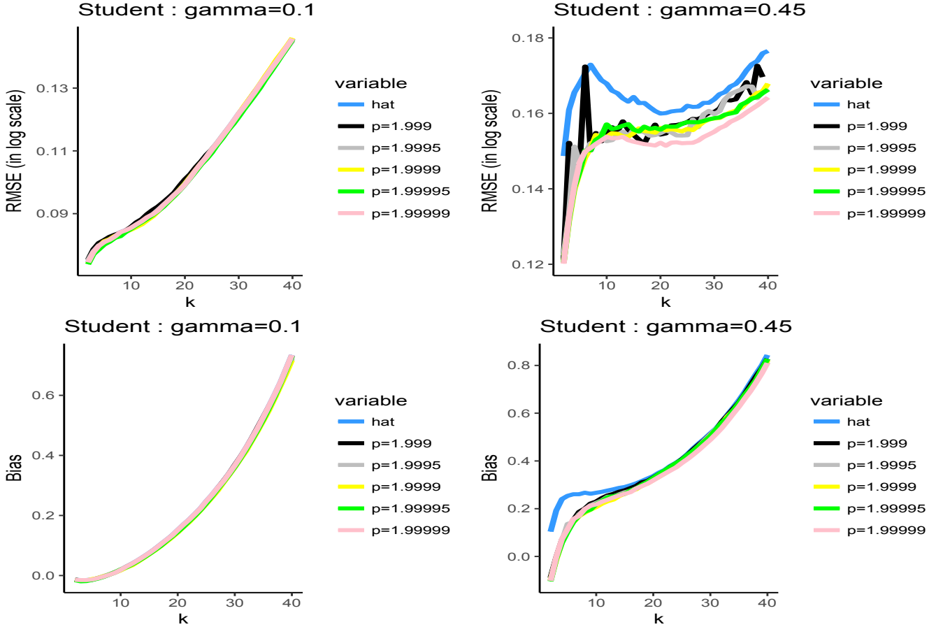
Figure 4: Student distribution. Top—RMSE (in log scale) of \hat{q}_{\tau'_n}^W(2) (blue) and \hat{q}_{\tau'_n(p, \alpha_n; 2)}^W(p) with p = 1.999 (black), p = 1.9995 (grey), p = 1.9999 (yellow), p = 1.99995 (green) and p = 1.99999 (pink). From left to right, \gamma = 0.1, 0.45 . Bottom—Bias estimates.
