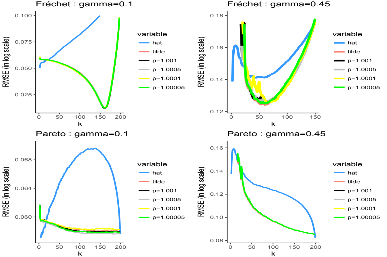
Figure 3: Fréchet and Pareto distributions—RMSE (in log scale) of \hat{q}_{\alpha_n}^W(2) (blue), \tilde{q}_{\alpha_n}^W(2) (red), and \hat{q}_{\hat{\tau}'_n(p, \alpha_n; 2)}^W(p) with p = 1.001 (black), p = 1.0005 (grey), p = 1.0001 (yellow) and p = 1.00005 (green). From left to right, \gamma = 0.1, 0.45 . From top to bottom, Fréchet and Pareto distributions .
