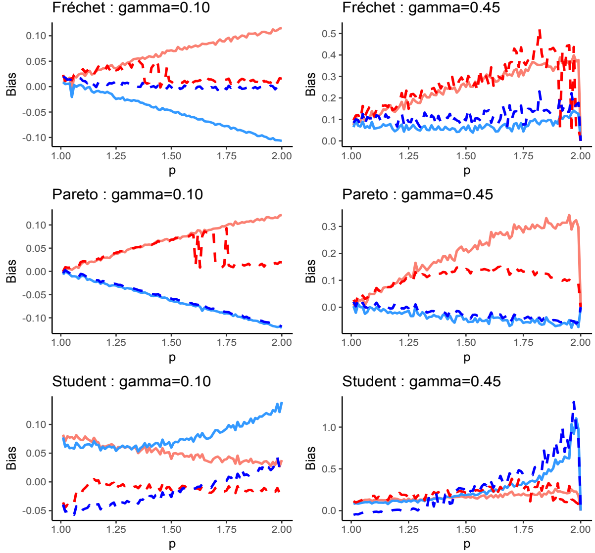
Figure 13: Bias estimates of \hat{q}_{\tau'_n}^W(p) in red and \hat{q}_{\tau_n}^W(p) in blue, as functions of p , with \tau'_n = 1 - 1/n . In solid lines the estimates obtained via the data-driven method, in dashed lines the estimates obtained via the RMSE minimization.
