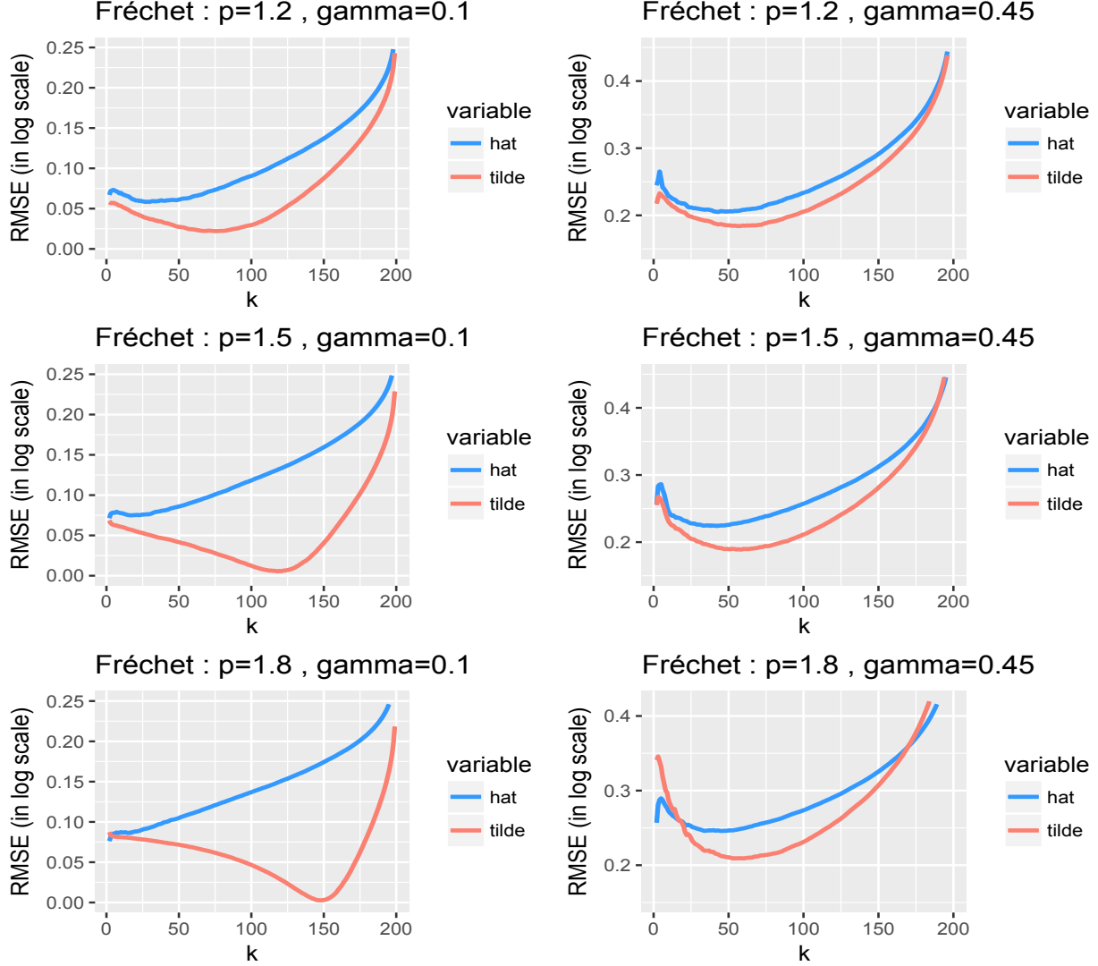
Figure 8: Fréchet distribution —RMSE (in log scale) of \hat{q}_{\tau'_n}^W(p) (blue) and \tilde{q}_{\tau'_n}^W(p) (red) as function of k \in \{2, \dots, n-1\} . From left to right, \gamma = 0.1, 0.45 . From top to bottom, p = 1.2, 1.5, 1.8 .
