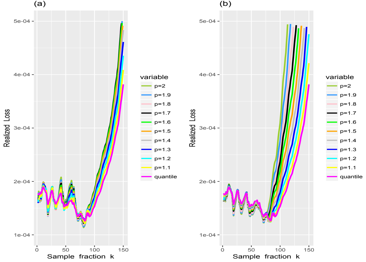
Figure 19: (a)—Plots of the realized loss k \mapsto \bar{L}_n^{(m)}(k) for \hat{q}_{1/n}^W(1) in magenta and \hat{q}_{\tau_n}^W(p) with different values of p . (b)—Results with \hat{q}_{\tau_n}^W(p) in place of \hat{q}_{1/n}^W(p) . Results based on weekly loss returns.
