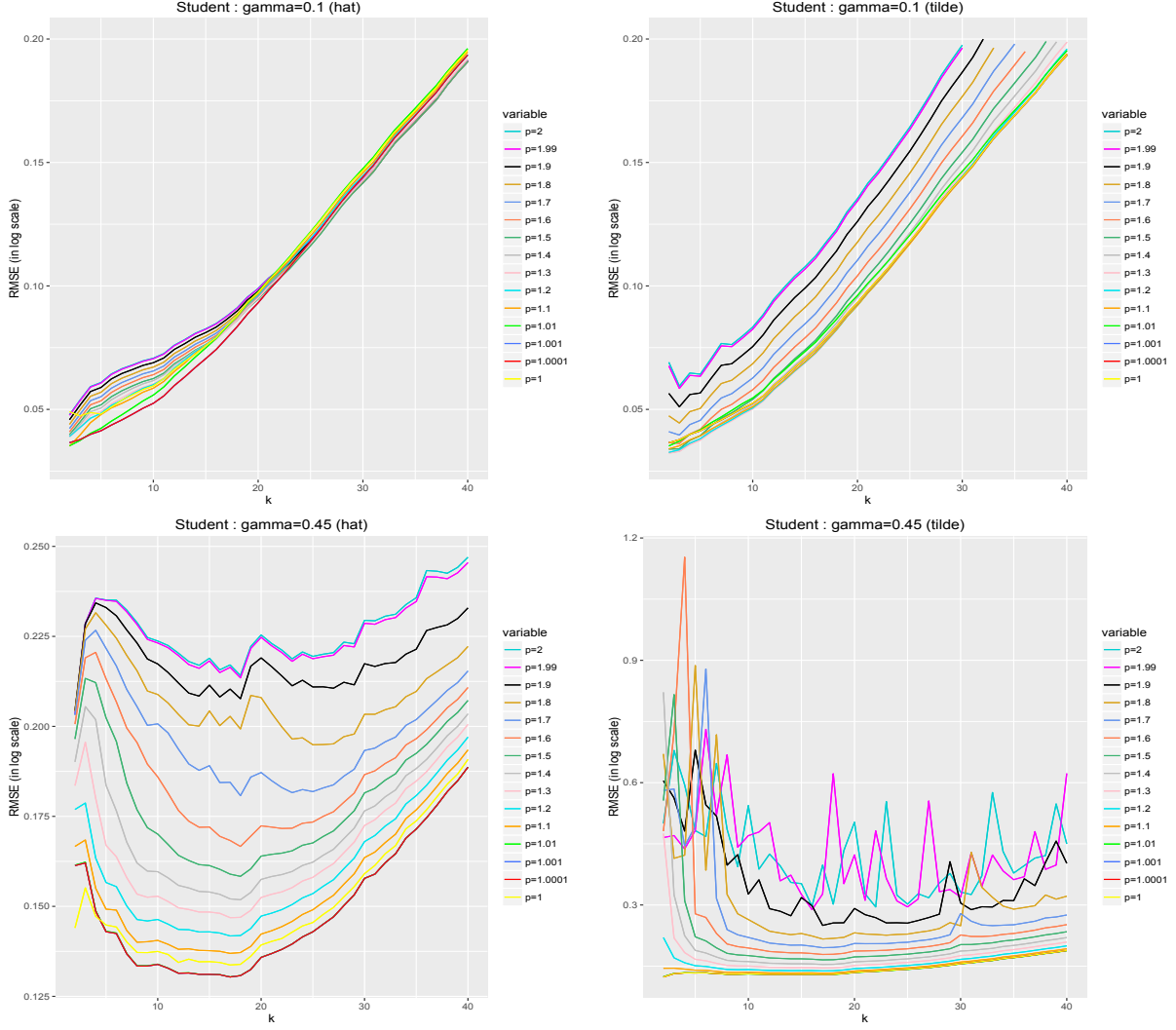
Figure 6: Student distribution —RMSE (in log scale) of \hat{q}_{\tau_n}^W(p) in left panels and \tilde{q}_{\tau_n}^W(p) in right panels. From top to bottom: \gamma = 0.1, 0.45 .
