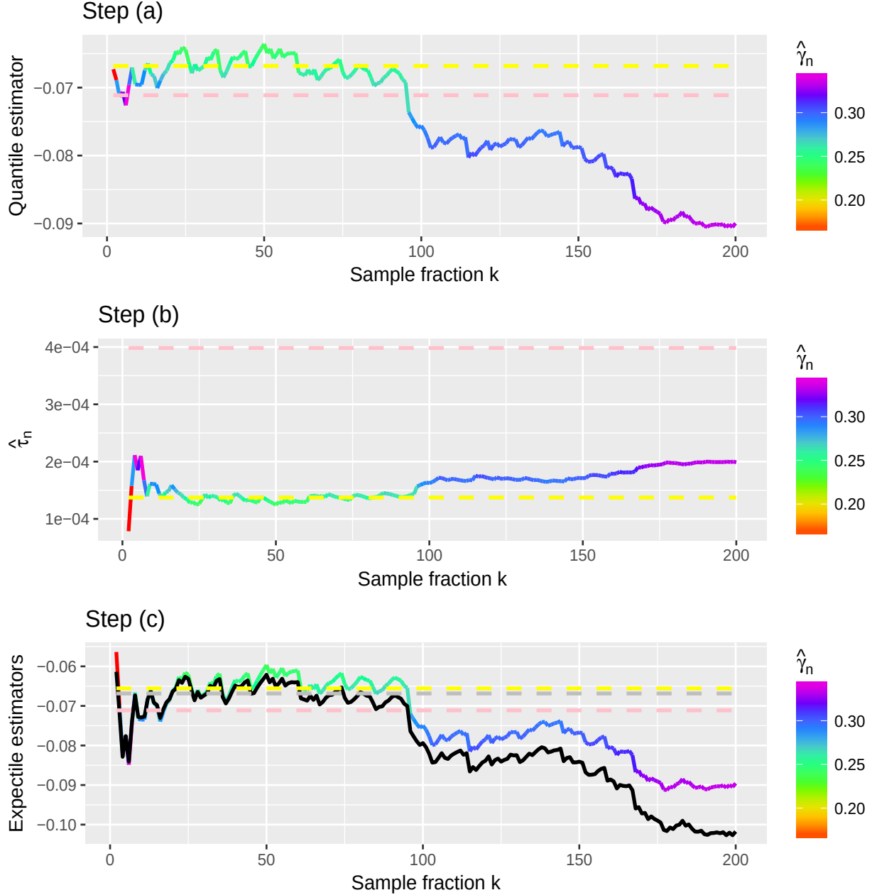
Figure 15: Step (a) —The plot of the estimator q_t^{(1)}(k) = \hat{q}_{1/n}^W(1) versus k as a rainbow curve. The selected optimal estimate q_t^{(1)}(\hat{k}_1) indicated by the horizontal yellow dashed line. The sample minimum log-return X_{1,n} indicated by the horizontal pink dashed line. Step (b) —The plot of the estimator \hat{\tau}'_n(p, k) , with p = 2 , versus k as a rainbow curve. The selected optimal estimate \hat{\tau}'_n(p, k) indicated by the horizontal yellow dashed line. The relative frequency 1/n indicated by the horizontal pink dashed line. Step (c) —The plots of the estimators q_t^{(2)}(k) = \hat{q}_{1/n}^W(p) and q_t^{(3)}(k) = \tilde{q}_{1/n}^W(p) versus k , respectively, as rainbow and black curves, with p = 2 . The selected optimal estimates q_t^{(2)}(\hat{k}_2) and q_t^{(3)}(\hat{k}_3) indicated, respectively, by the horizontal yellow and grey dashed lines. The minimum log-return X_{1,n} indicated by the horizontal pink dashed line. The effect of \hat{\gamma}_n(k) on q_t^{(2)}(k) is highlighted by the colour-scheme.
