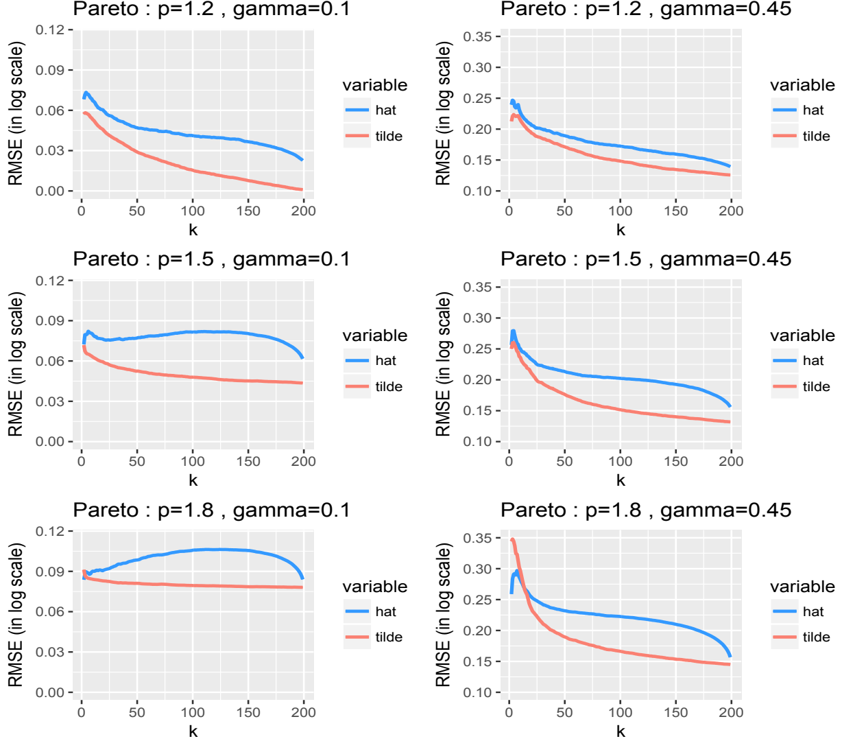
Figure 9: Pareto distribution —RMSE (in log scale) of \hat{q}_{\tau'_n}^W(p) (blue) and \tilde{q}_{\tau'_n}^W(p) (red) as function of k \in \{2, \dots, n-1\} . From left to right, \gamma = 0.1, 0.45 . From top to bottom, p = 1.2, 1.5, 1.8 .
