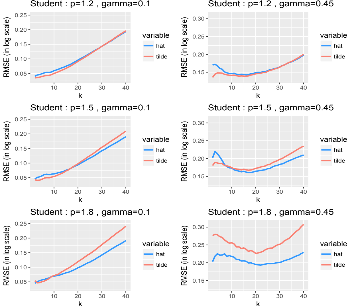
Figure 10: Student distribution—RMSE (in log scale) of \hat{q}_{\tau'_n}^W(p) (blue) and \tilde{q}_{\tau'_n}^W(p) (red) as function of k . From left to right, \gamma = 0.1, 0.45 . From top to bottom, p = 1.2, 1.5, 1.8 .
