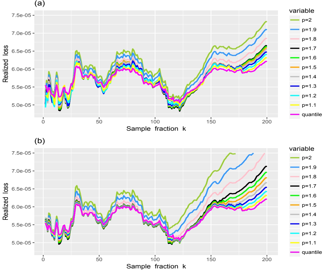
Figure 17: (a)—Plots of the realized loss k \mapsto \bar{L}_n^{(m)}(k) for \hat{q}_{1/n}^W(1) in magenta and \hat{q}_{\tau_n}^W(p) with different values of p . (b)—Results with \tilde{q}_{\tau_n}^W(p) in place of \hat{q}_{\tau_n}^W(p) . Results based on daily loss returns.
