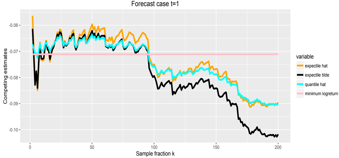
Figure 16: The plots of the three estimators q_t^{(1)}(k) = \hat{q}_{1/n}^W(1) in blue, q_t^{(2)}(k) = \hat{q}_{\tau'_n}^W(2) in orange, and q_t^{(3)}(k) = \tilde{q}_{\tau'_n}^W(2) in black. The sample minimum X_{1,n} in pink.
