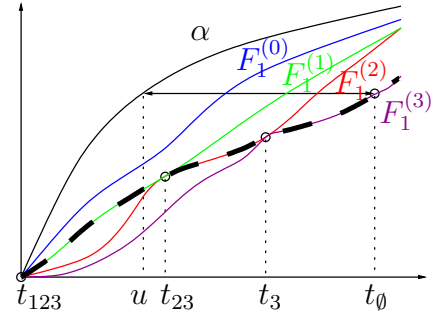
Fig. 3. Reading t_\pi on a trajectory for a 1-flow 3-servers scenario.
