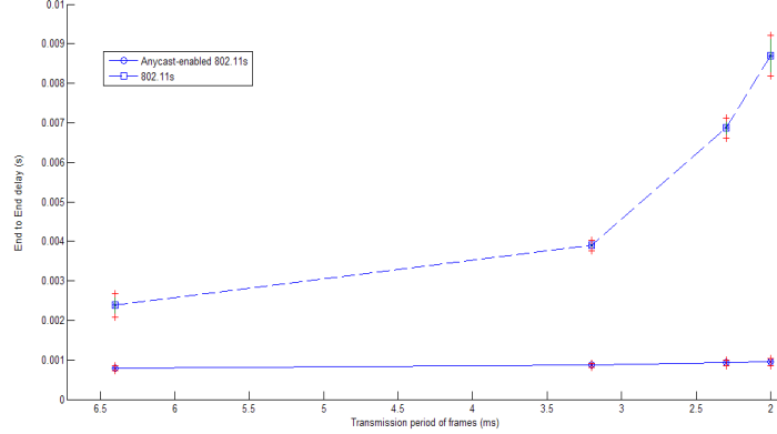
Fig. 6. End-to-End delay versus the transmission period for Internet and intra-mesh traffic.
