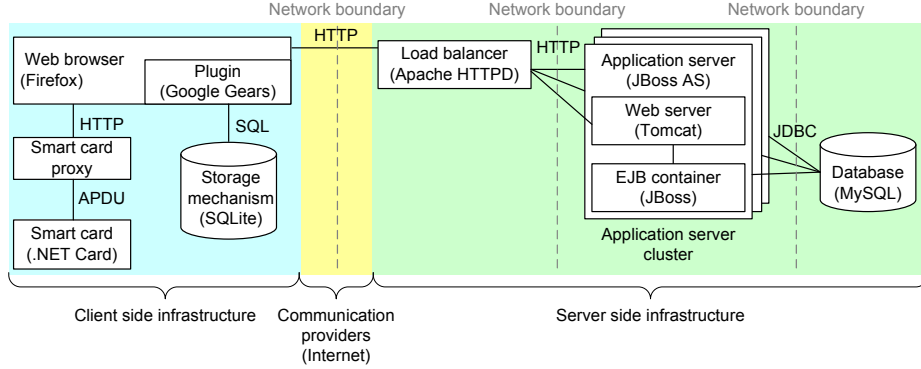
Fig. 1. Prototype architecture
