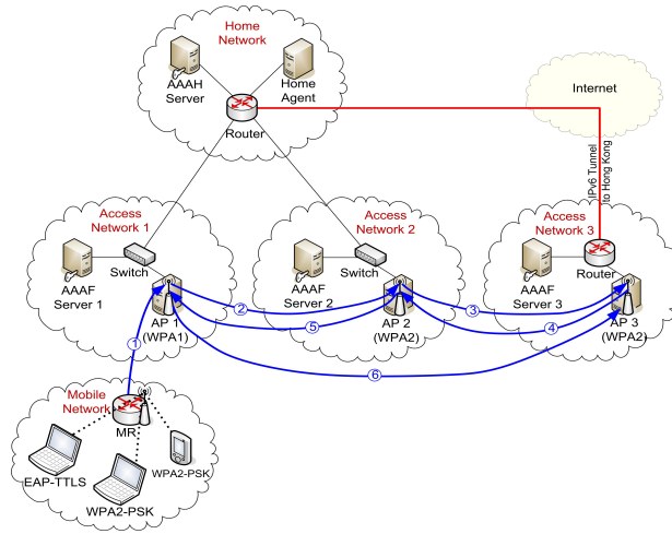
Fig. 2. Experimental Testbed
