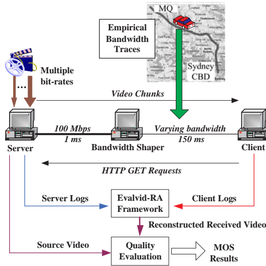
Fig. 3. Experiment setup
