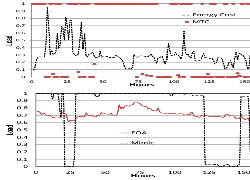
Fig. 3: Job load and normalized electricity price over time at Boston, MA. The top graph shows the electricity price and the load that MTC puts on this DC. The bottom graph shows the load for EOA and MimicOPT.
