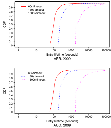
Fig. 8. Cumulative Distribution Function of entries' lifetime.
