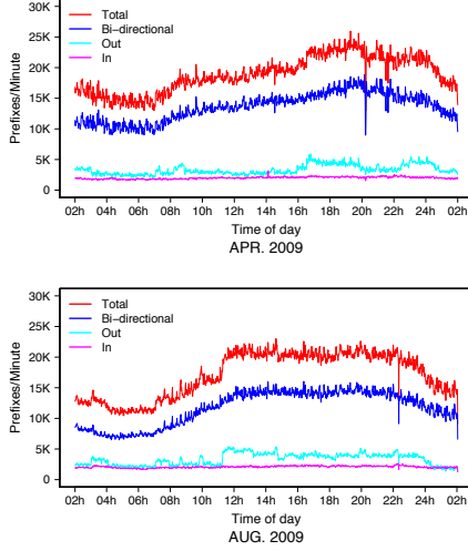
Fig. 3. Report of the number of correspondent prefixes per minute.
