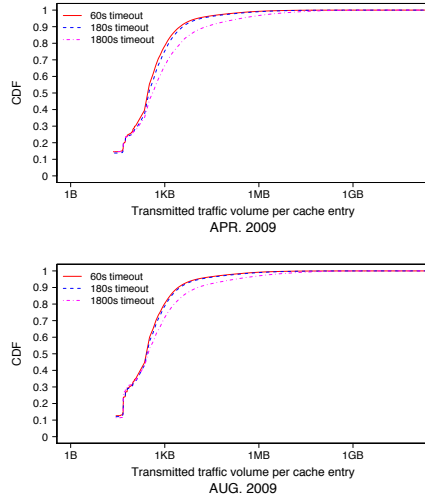
Fig. 7. Cumulative Distribution Function of the traffic volume per cache entry.
