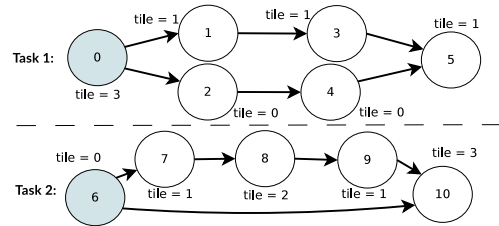
Fig. 16: Two DAGs
