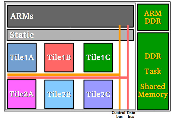
Fig. 7: FPGA device
