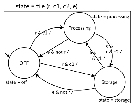
Fig. 10: Reconfigurable tile
