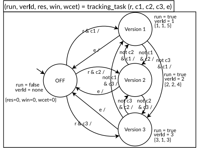
Fig. 17: Automata-based model for the tracking task
