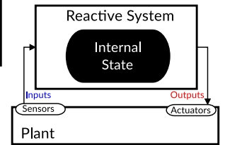
Fig. 2: Reactive system
