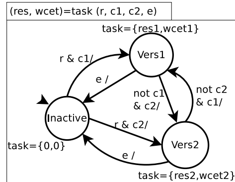
Fig. 11: Computation task
