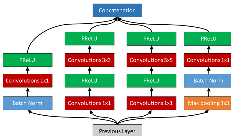
Fig. 1 Modified Inception module using PReLU and Batch Normalization
