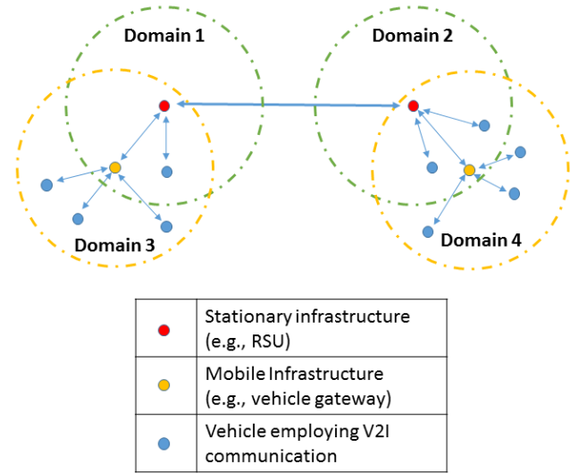
Fig. 2. Controller Domains
