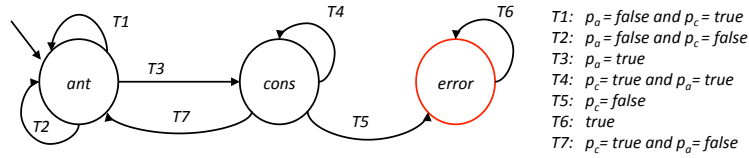
Fig 6: Example of the checker for assertion always(p_a \rightarrow next(p_c)) .
