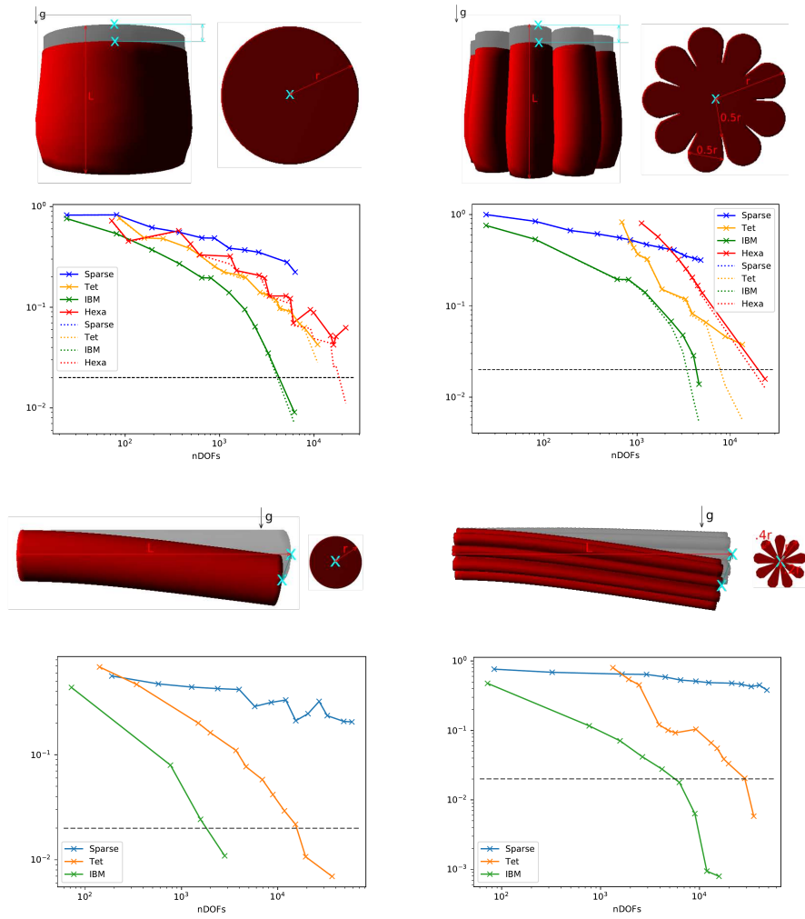
Fig. 2 Compression ( top ) and bending ( bottom ) example with different cross sections ( left/right ): Top : Setup of the example in front ( left ) and top ( right ) view with the initial ( grey ) and final ( red ) configuration of the beam and the point at which we measure the distance in turquoise ; Bottom : Convergence analysis, with the comparison of only the z values as dashed curves and the dashed black line depicts a relative error of 2%.
