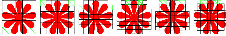
Fig. 4 Bending example: Several chosen resolutions of simulations with a regular hexahedral topology, showing the two-dimensional cross section with the grid: for the sparse grid, all displayed elements are simulated as completely filled, while for the IBM green elements are deleted (since they have less than 5% of the hexahedral volume) and boundary elements are partially filled.
