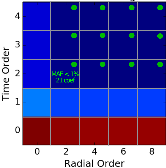
Gaussian Fitting
