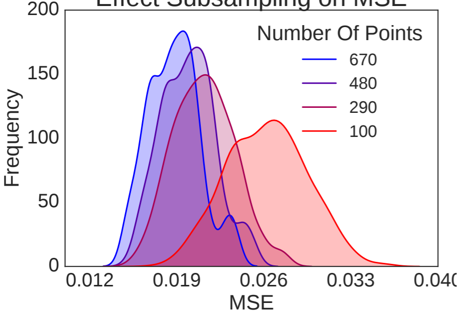
Effect Subsampling on MSE
