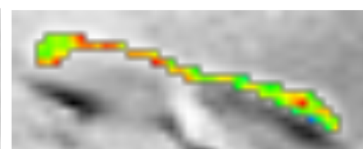
Effect Subsampling on RTOP
