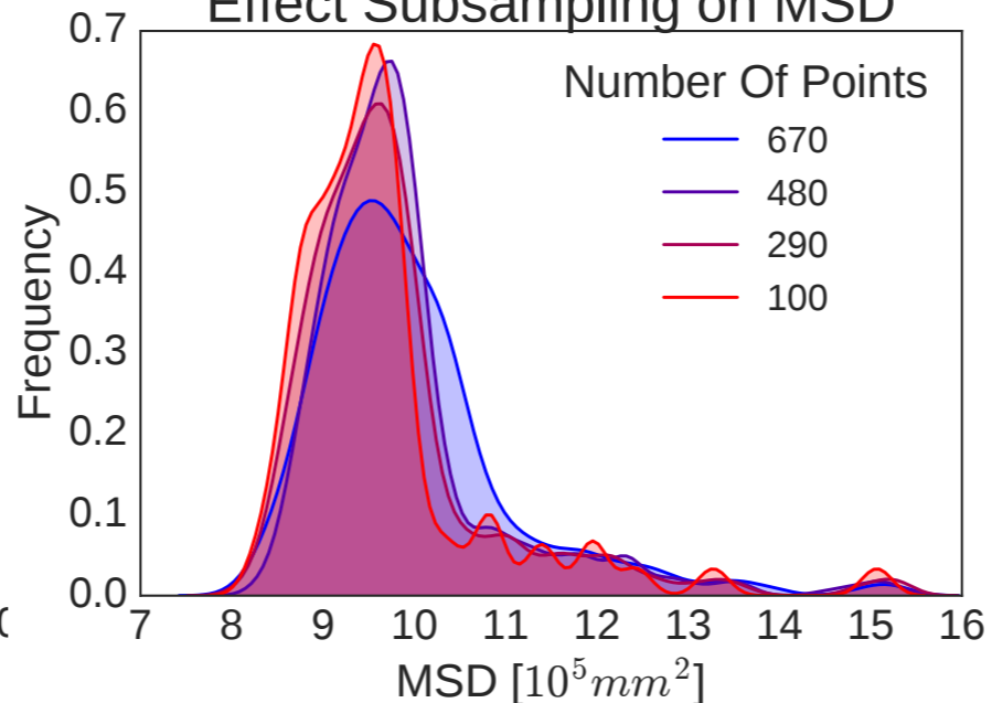
Effect Subsampling on MSD
