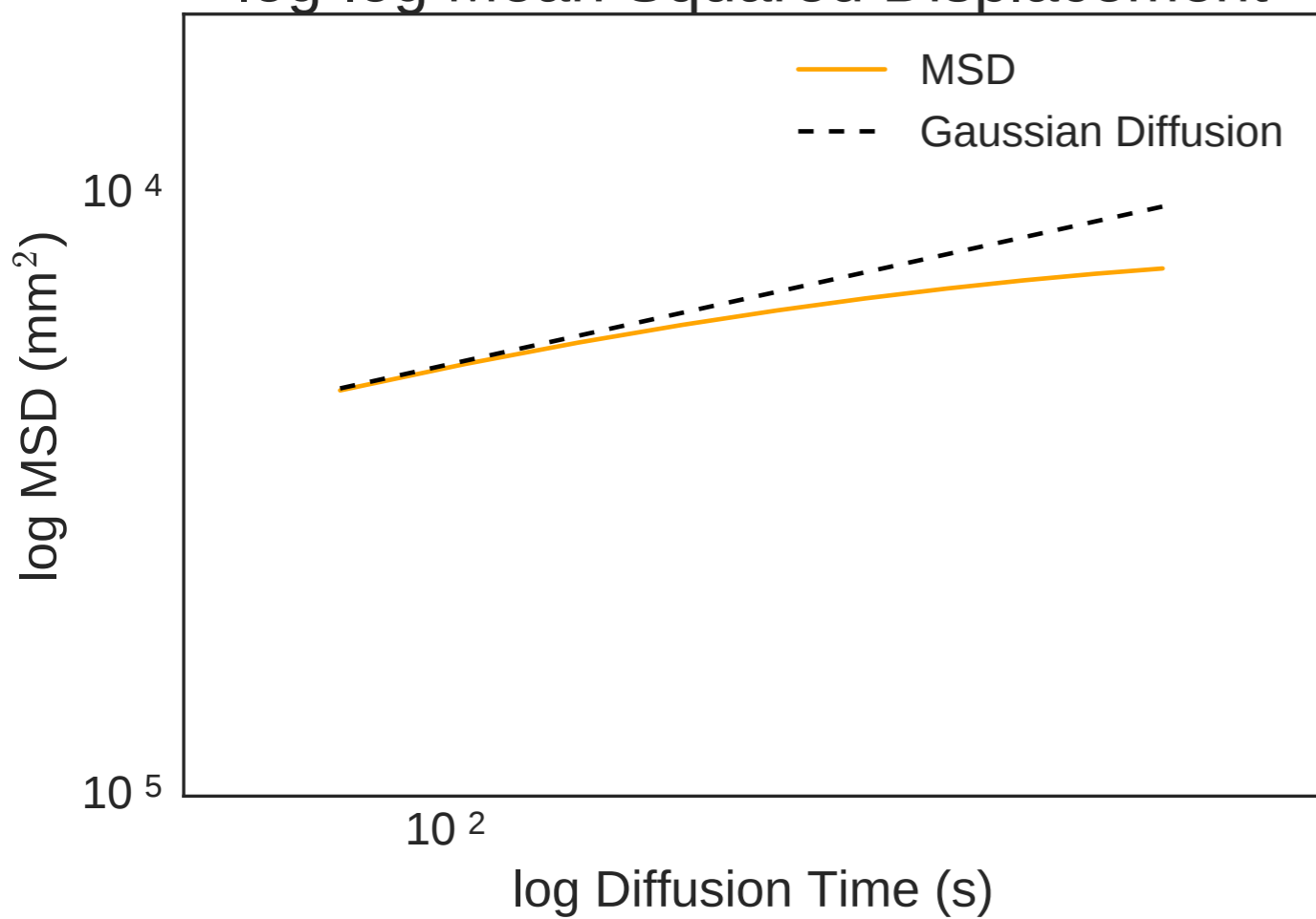
log log Mean Squared Displacement
