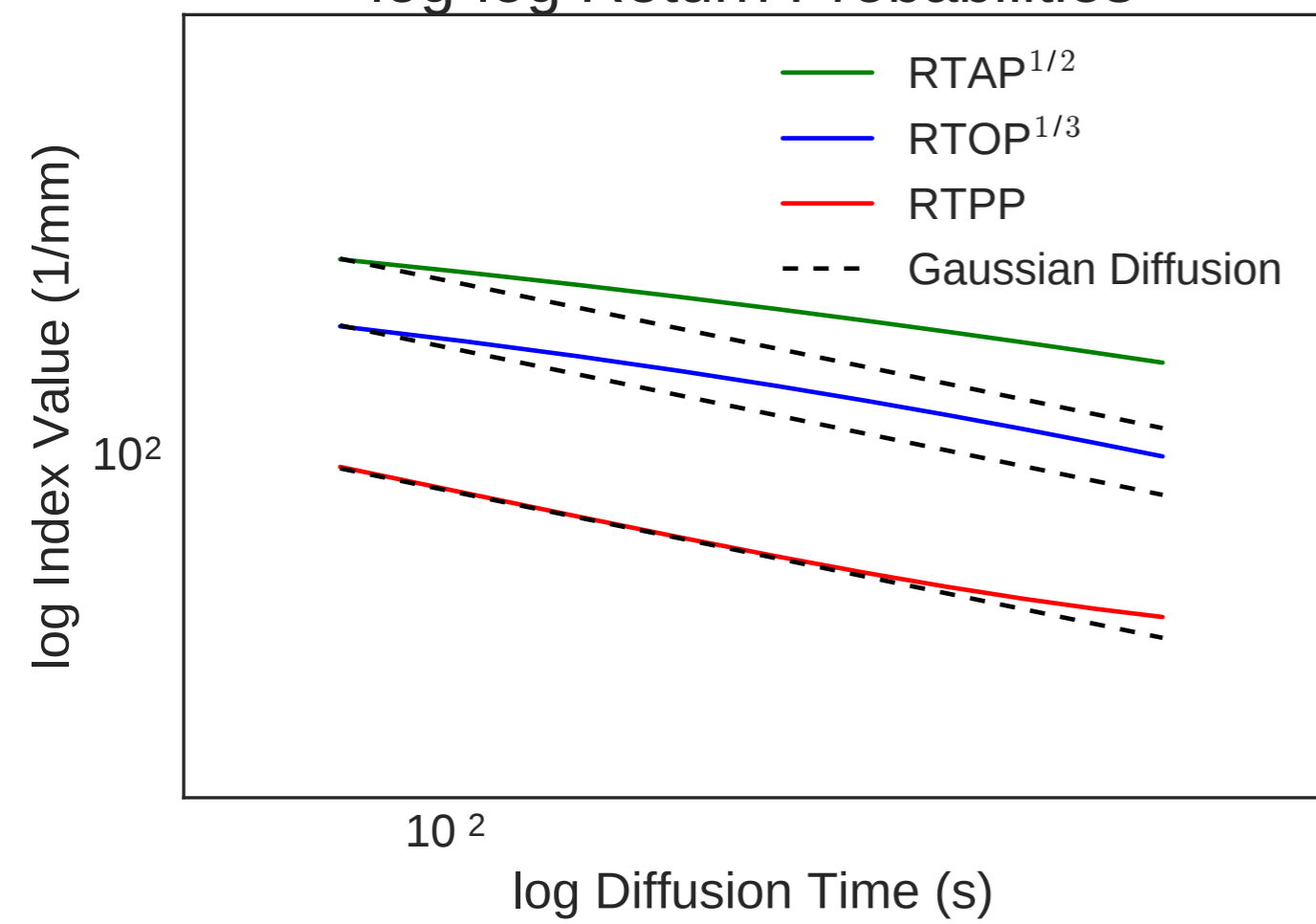
log log Return Probabilities
