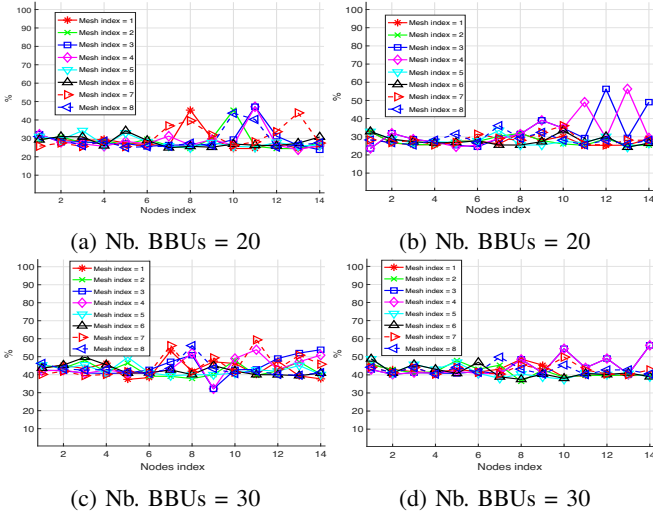
Fig. 5: Resource utilization for every node; Homogeneous index = 1 and 5 for 5a, 5c, and 5b, 5d, respectively
