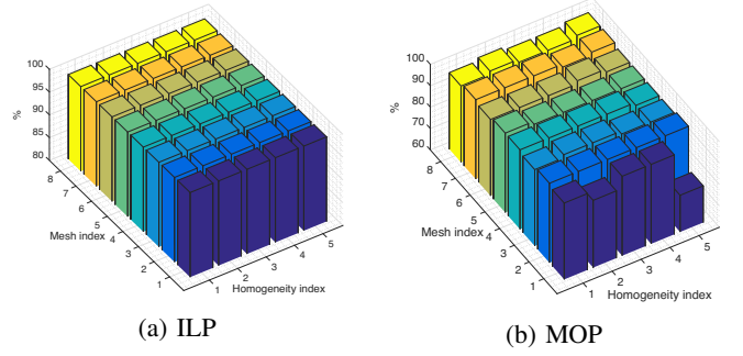
Fig. 3: Acceptance Ratio
