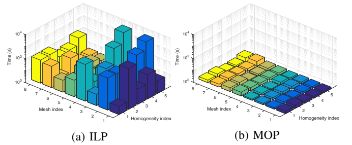
Fig. 4: Embedding time
