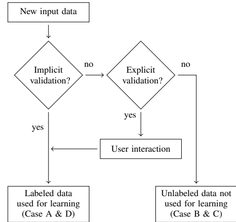
Figure 4: Online active learning supervision process.
