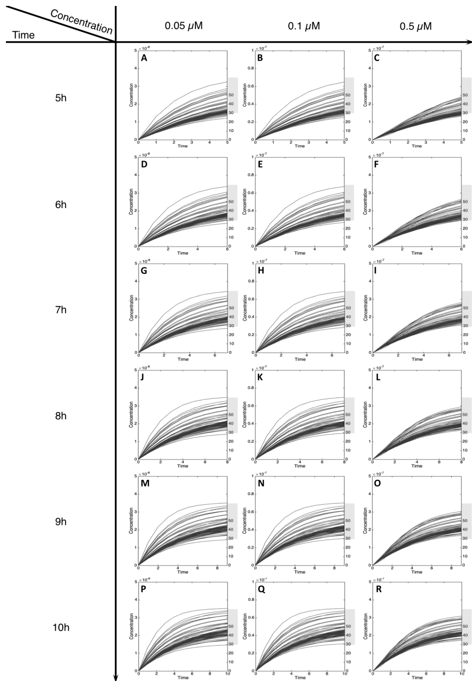
Figure 5 Metabolism of C-Hydroxy-MeIQx at initial concentration of 0.05, 0.1, 0.5 \mu\text{M} after 5, 6, 7, 8, 9, 10 h of exposition. The grey rectangle represents the area between 30 and 70% of the MeIQx metabolized. Concentrations are in Molar on the y axis and time in hours on the x axis. (A, D, G, J, M, P) C-Hydroxy-MeIQx formation at an initial MeIQx concentration of 0.05 \mu\text{M} (B, E, H, K, N, Q) C-Hydroxy-MeIQx formation at an initial MeIQx concentration of 0.1 \mu\text{M} (C, F, I, L, O, R) C-Hydroxy-MeIQx formation at an initial MeIQx concentration of 0.5 \mu\text{M} .
