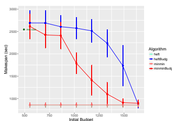
(j) Cyber, 90 tasks, \sigma = 1.0
