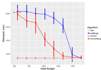
(g) Cyber, 90 tasks, \sigma = 0.75
