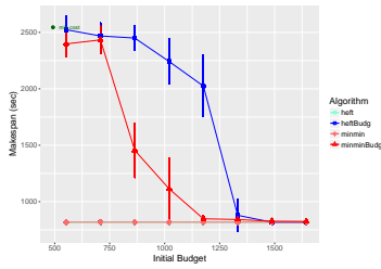
(a) Cyber, 90 tasks, \sigma = 0.25
