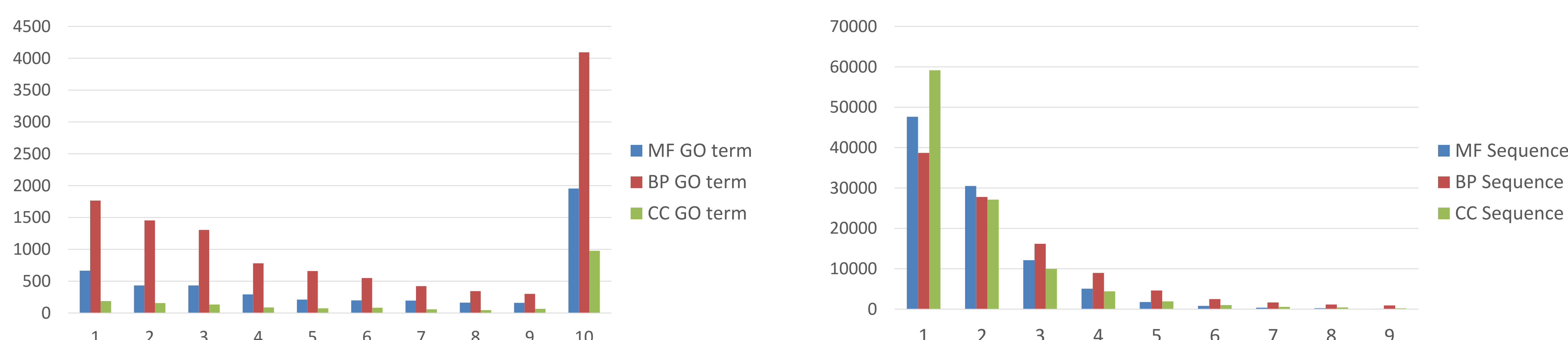
Fig2. CAFA3: Distribution according to the number of GO terms for each sequence (right), and sequences for each GO term (left)
