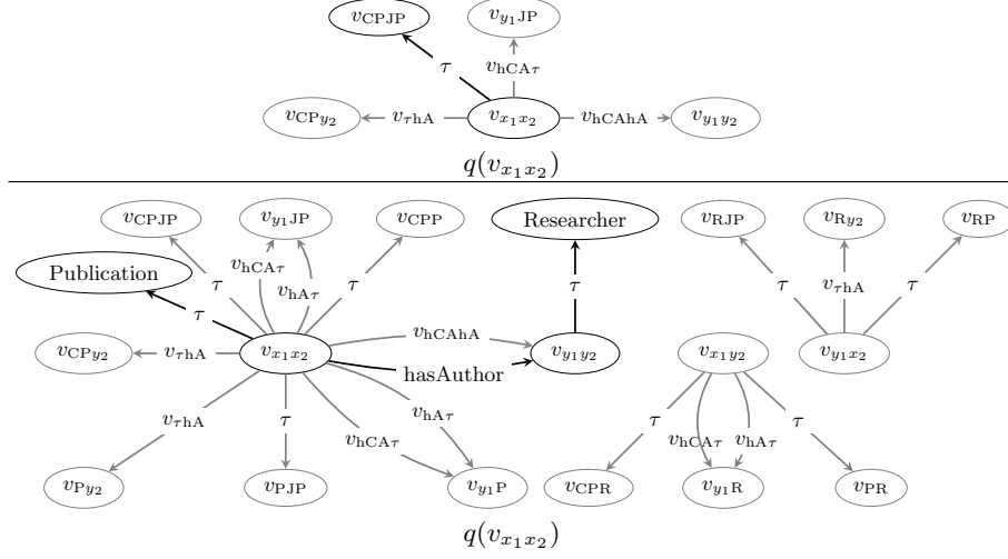
Fig. 5: Cover queries of the BGPQs q_1 and q_2 in Figure 3 (top) and of their saturations q_{1\mathcal{O}} and q_{2\mathcal{O}} in Figure 4 (bottom). Triples in grey are redundant w.r.t. those in black.
