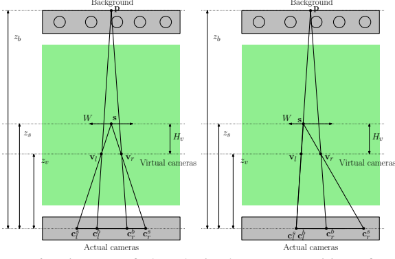
Figure 6. Diagram of the obtained camera positions for the “Quadri-Rig”. Left: the cameras acquiring the subject c_s^* are aligned with the position of the subject of interest s and the virtual cameras c_s^v . The cameras acquiring the background c_b^* are aligned with the center of the background p and the virtual cameras c_b^v . Right: When s , p and v_l are aligned, c_l^b and c_l^s are equal.
