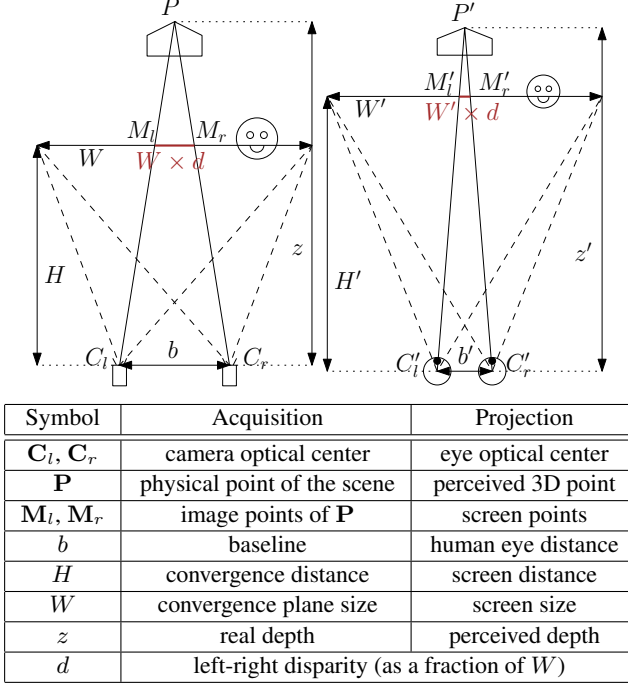
Figure 1. Parameters describing the shooting and projection geometries (reproduced from [10]). ( l and r indicate left and right).
