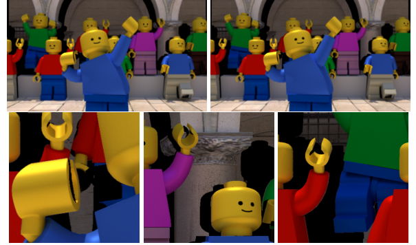
Figure 12. First row: stereoscopic pair obtained from the Quadri-Rig with [33]. Second row: closeups of the rendered views. As the background is not a plane, large areas in black are not acquired by any actual camera (compare with Fig. 15).
