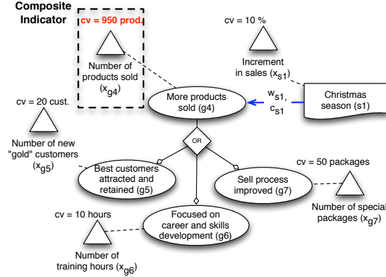
Fig. 5. Examples of reasoning with conversion factors: cv = current value, w = weight, c = conversion factor.
