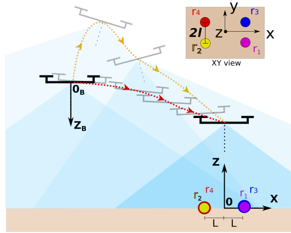
Fig. 2. Consider two pairs of dots on the ground horizontal plane (XY view in the upper right corner). It would be possible to cope with the field of view constraints by planning a near hovering trajectory (e.g. path in red), but in this work we aim at finding a trajectory similar to the path in yellow which is much more dynamic (and with a shorter completion time).
