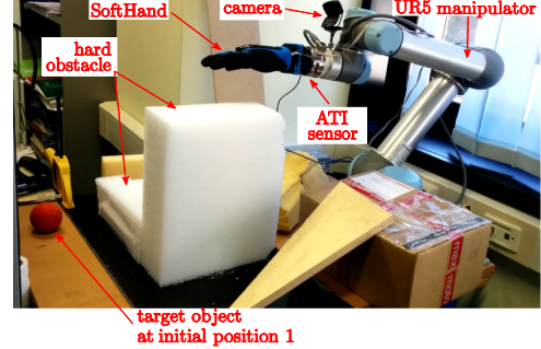
(b) Remote environment with hard obstacles between the slave robot and the target object to grasp.
