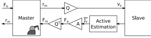
Fig. 2: The teleoperation architecture. The active estimation block computes the direction to track \tilde{J}_v and A = k \left( I_2 - \frac{v_s v_s^T}{v_s^T v_s} \right) projects it in the null space of the velocity of the slave.
