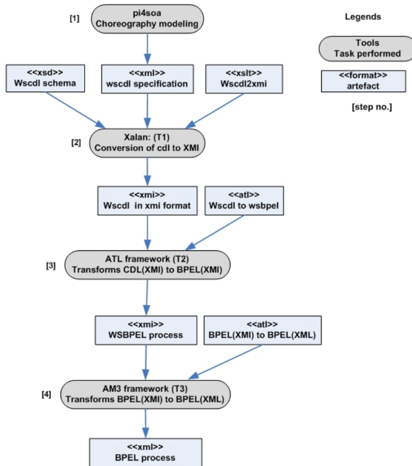
Fig. 4. Transformation Chain
