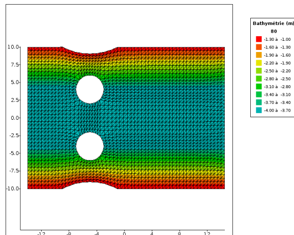
Figure 6: Mesh and bathymetry of the bridge piers test case.
