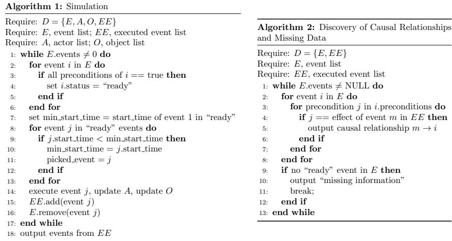
Figure 8. Key algorithms.
