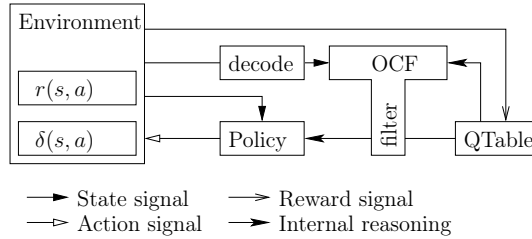
Fig. 2. Two-level reinforcement learning set-up. The ranking function (“OCF c ”) acts as a filter on the possible actions a reinforcement learning agent may take.
