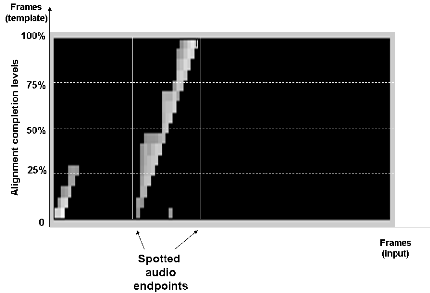
Fig. 4. Pattern matching executed by sliding along the whole audio stream to find best alignment of the template (audio pattern to be spotted) into the audio stream (input).
