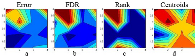
Fig. 2. Evaluation of the FDR, Rank and Centroids measures against their ability to predict the performance of the linear readout map of an LSM. In each subplot the x,y axes correspond to different configurations for an LSM. The color in each x,y entry corresponds to the value of the error (for subplot a) or the negative value of the measure (for subplots b,c,d).
