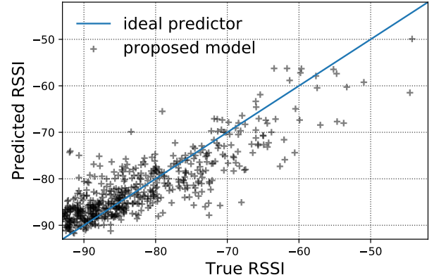
Fig. 6. RSSI predictor accuracy compared to an ideal predictor (blue line) on the testing dataset of 555 RSSI measurements.
