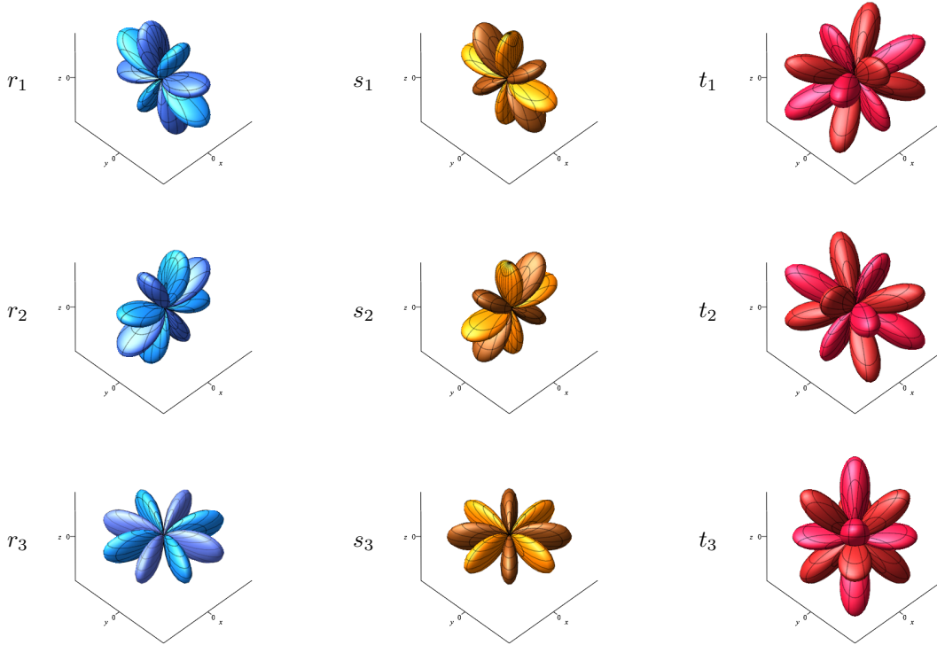
FIGURE 4.1. Harmonic quartics
