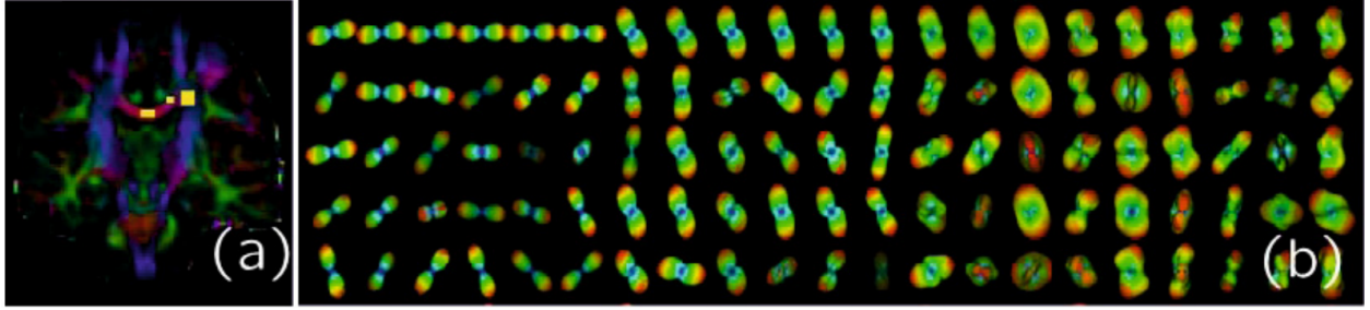
FIGURE 1.2. Slice of a brain diffusion image (a). The yellow boxes indicate the regions that are zoomed in (b) showing the individual voxel shapes. From [PGD14].
