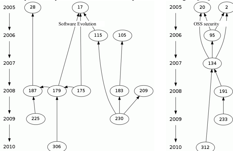
Fig. 5. Clusters #17 and #20_2
