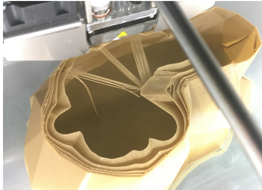
Figure 3: An unusually high number of bridges appears during the printing of the Fawn model.
