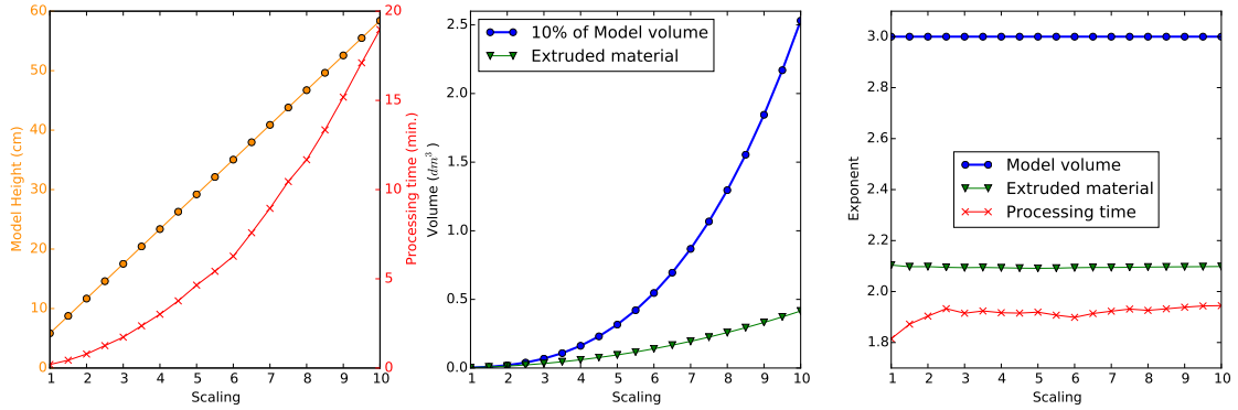
Figure 5: The horizontal axis is the scaling factor applied to the input model. Left . Height of the model and processing time, including loading the STL file, processing the slices and writing the GCode file. Middle . Volume of the input model (divided by 10 for clarity) and volume of the extruded material for printing the modeling with our cavities. Right . Estimation of the exponent \alpha when approximating the curves in Left and Middle with a formula of type Rs^\alpha where R is a constant. s is the scaling factor (in abscissa). As expected, the exponent is exactly 3 for the volume. It is just above 2 for the volume of extruded material, which indicates that the volume of our cavities walls scales more like a surface than like a volume.
