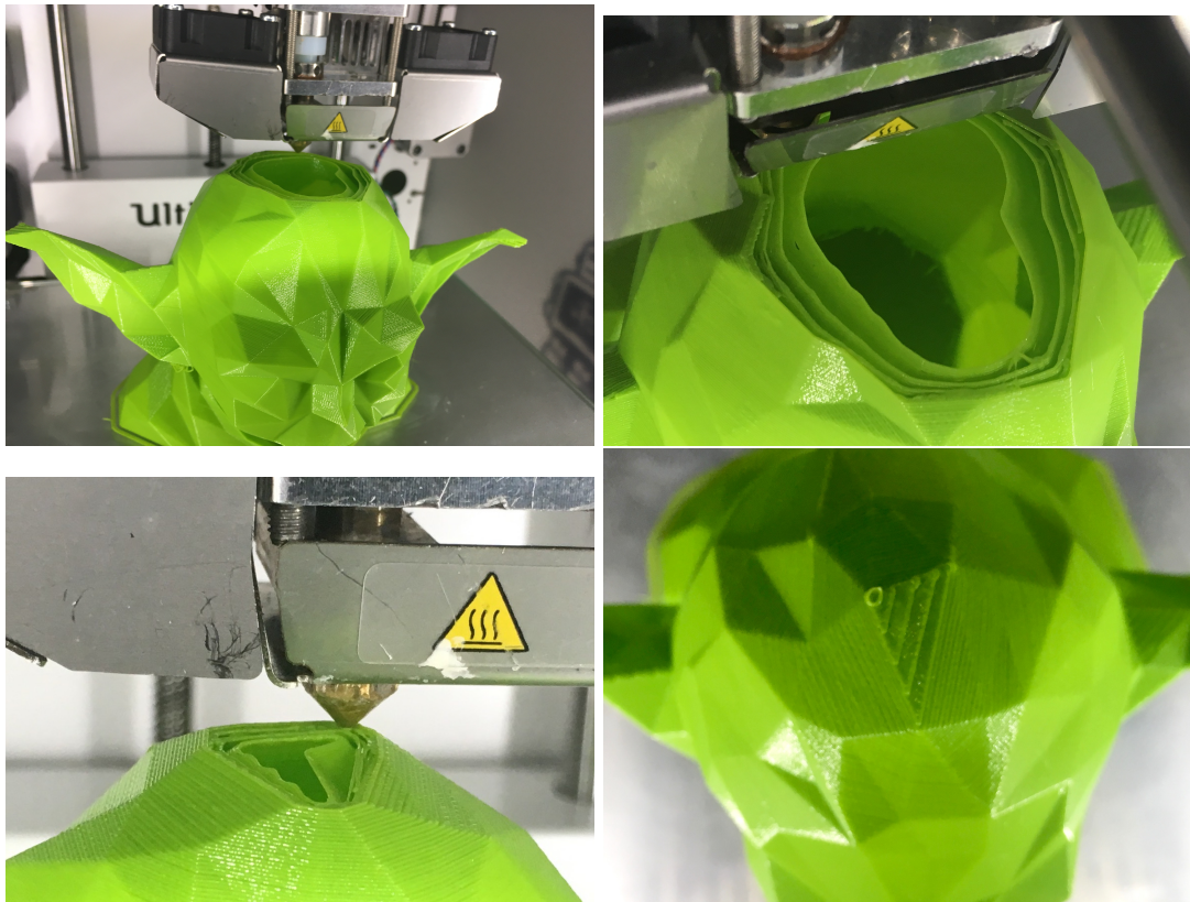
Figure 4: Timelapse of the printing of a Yoda model. ( Top-right. ) Note how the print is mostly empty and the nested cavity walls. Bottom-left. Approaching the top of the head. Bottom-right. Closing the top of the head.
