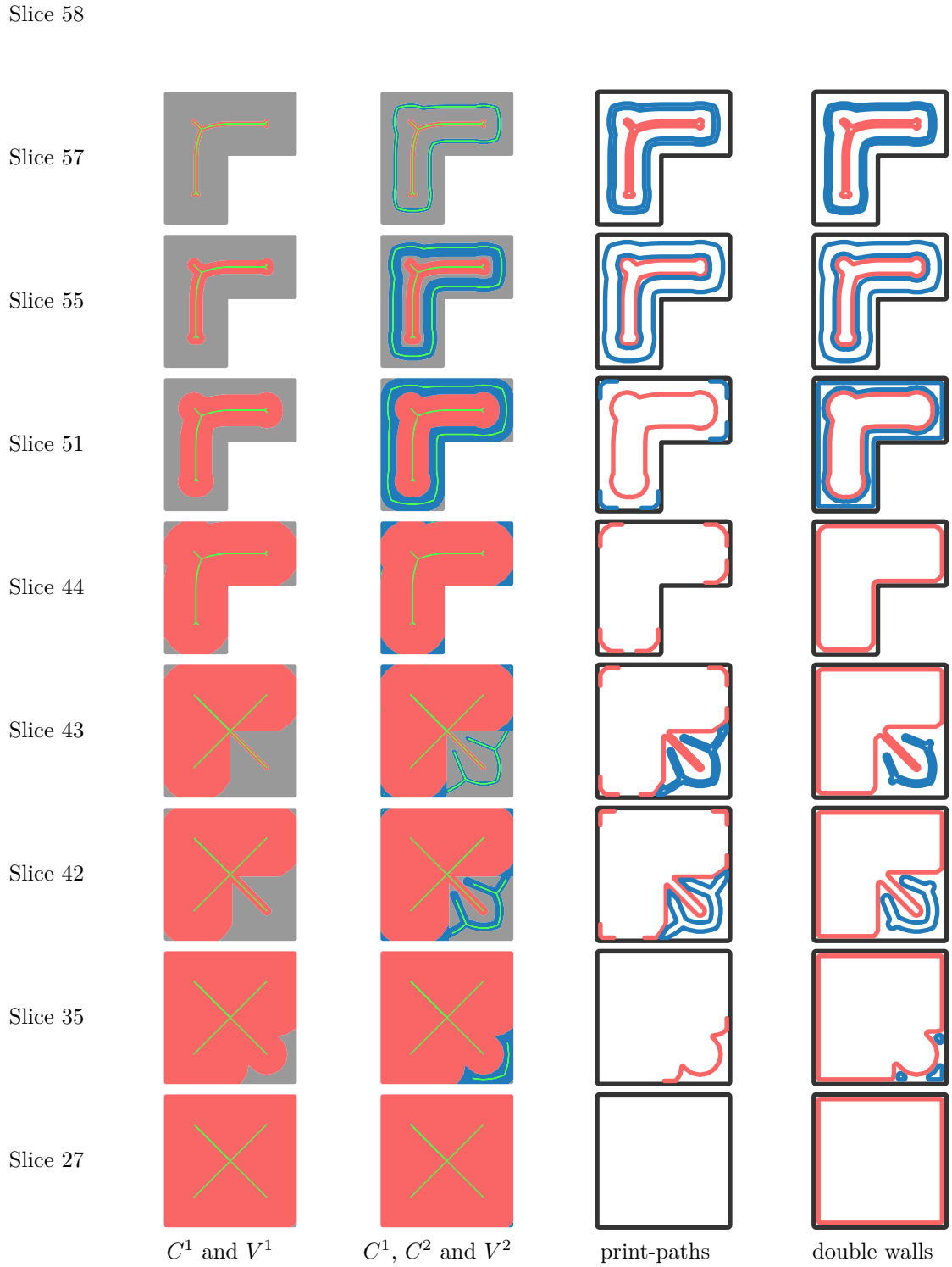
Figure 2: An example of modeling cavities with two iterations. Same color scheme as Figure 1.
