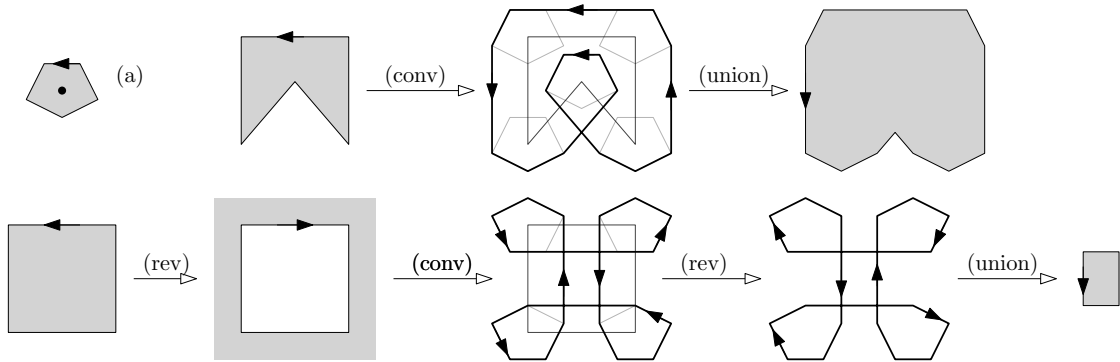
Figure 2: Computing the Minkowski sum between a general polygon and a convex structuring element. Top. (a) The structuring element, with its reference point. For a dilation , we first (conv)olve the contour(s) of the general polygon with the contour of the structuring polygon. We then compute the (union) of the convolved contours using the Clipper library. Bottom. For an erosion , we (rev)erse the contours of the general polygon (which is akin to taking the complement), (conv)olve them with then contour of the center symmetrical structuring polygon, and (rev)erse the resulting contour. Finally, we compute the (union) as above.
