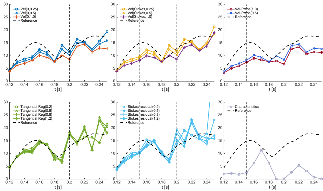
Figure 33. Benchmark 2 (stenosis), air regime: incoming flow rate [\text{cm}^2/\text{s}] over time [\text{s}] . The curves are shown starting from t = 0.12 s. Before this instant, the different methods yield very similar results.
