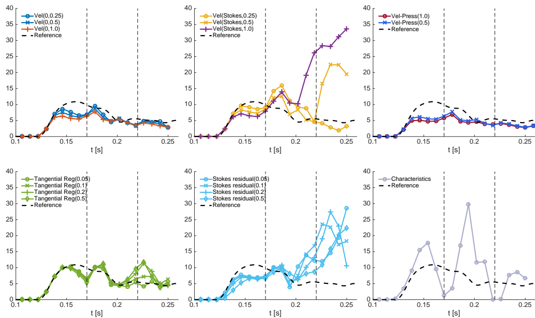
Figure 25. Benchmark 2 (stenosis), blood regime: incoming flow rate [ \text{cm}^2/\text{s} ] over time [s]. The curves are shown starting from t = 0.10 s. Before this instant, the different methods yield very similar results.
