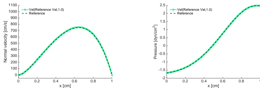
Figure 13. Profiles of velocity (left) and pressure (right) at the inflow boundary (peak backflow, t = 0.95 s), using an open boundary stabilization based on a velocity penalization towards the reference velocity (Benchmark 1, air regime).
