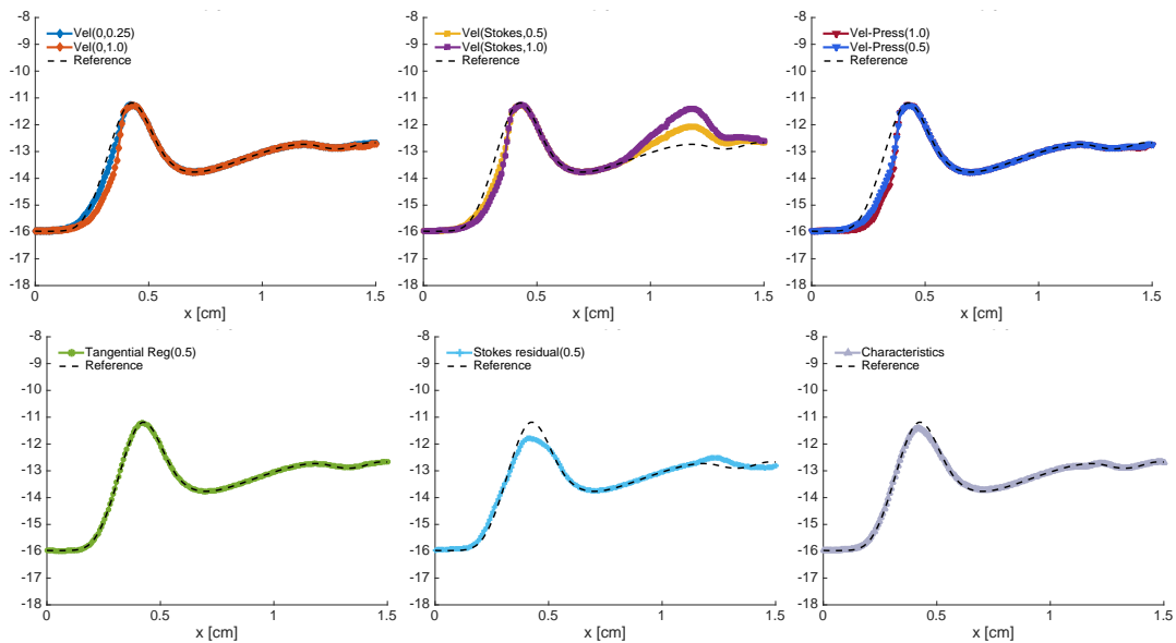
Figure 38. Benchmark 2 (stenosis), air regime (time t = 0.2 s): Pressure profiles along the open boundary [ \text{dyn}/\text{cm}^2 ].
