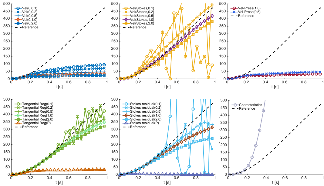
Figure 14. Benchmark 1 (full backflow), air regime: incoming flow rate [ \text{cm}^2/\text{s} ] over time [s].
