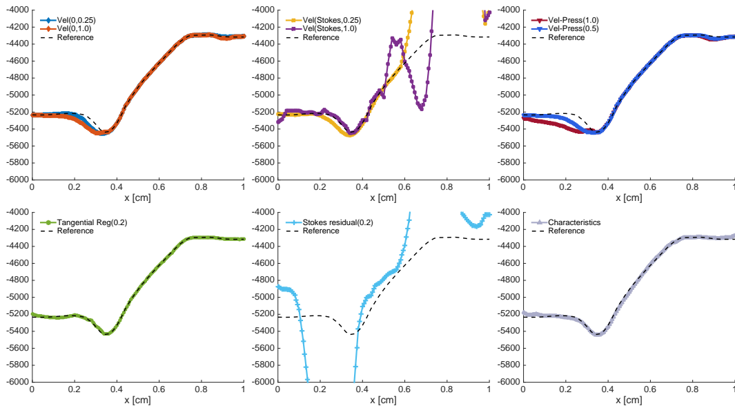
Figure 30. Benchmark 2 (stenosis), blood regime (time t = 0.32 s): Pressure profiles along the open boundary [dyn/cm 2 ].
