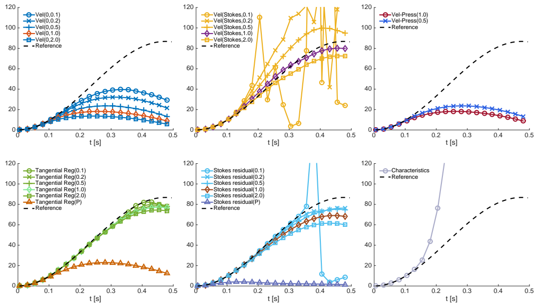
Figure 4. Benchmark 1 (full backflow), blood regime: incoming flow rate [ \text{cm}^2/\text{s} ] over time [s].
