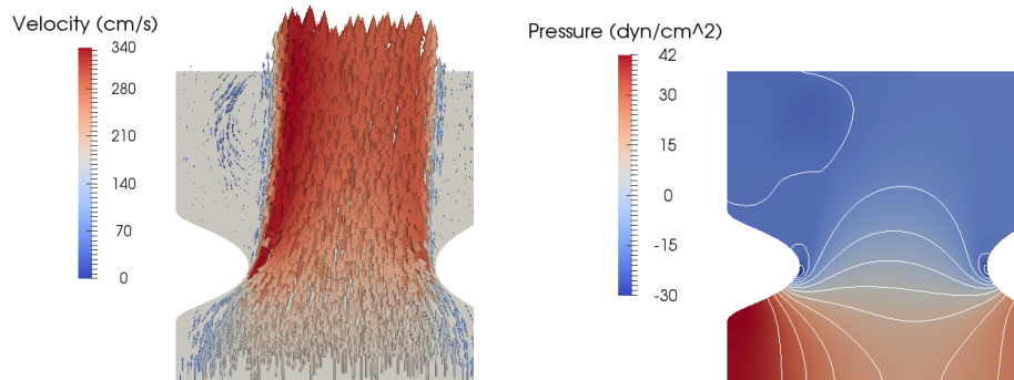
Figure 31. Benchmark 2 (stenosis), air regime. Reference solution at t=0.20 s. Left: Mesh and glyph vector of the velocity field. Right: Pressure isolines.
