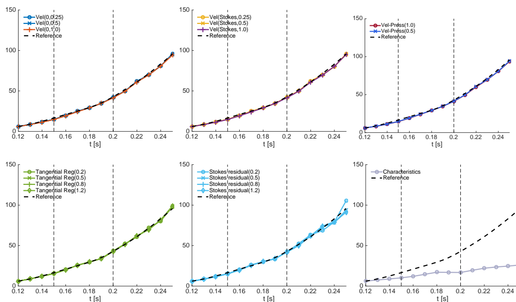
Figure 34. Benchmark 2 (stenosis), air regime: Average pressure drop [dyn/cm 2 ] over time [s]. The curves are shown starting from t = 0.12 s. Before this instant, the different methods yield very similar results.
