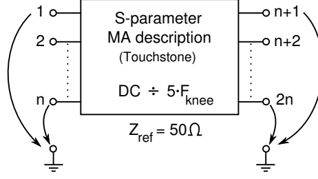
Fig. 7. Associated n-port model for an n -wire segment.
