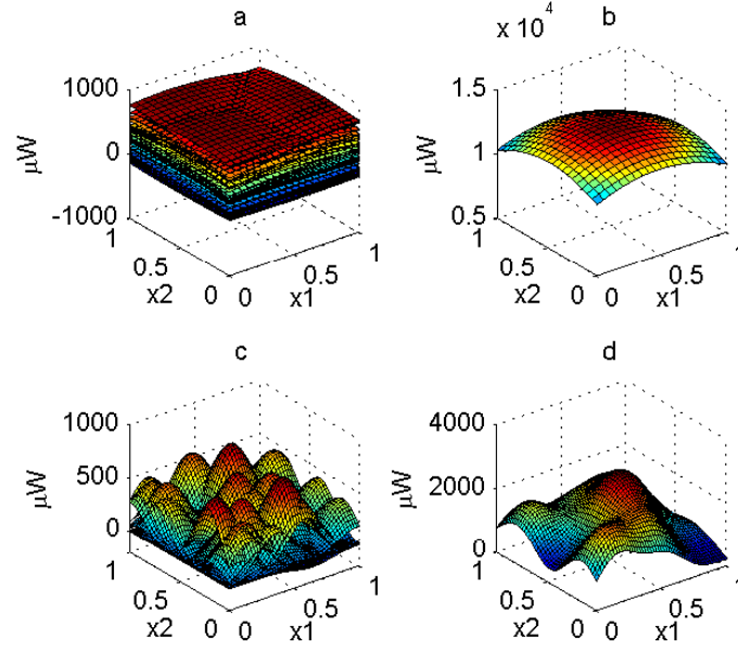
Fig. 4. Power surfaces for: a) \sigma = 1 , components; b) \sigma = 1 , sum; c) \sigma = 0.02 , components; d) \sigma = 0.02 , sum.
