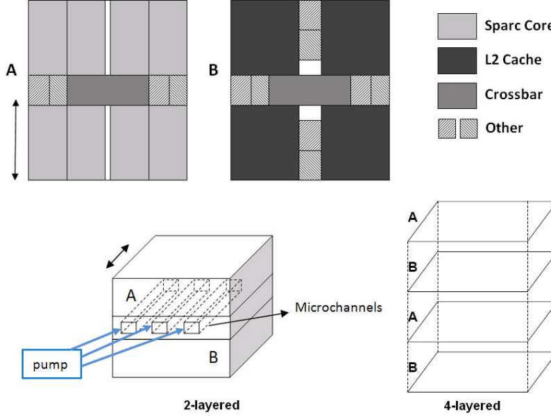
Fig. 4. Floorplans of the 3D Systems.
