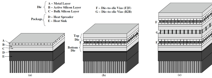
Fig. 2. Die-bonding process [31].
