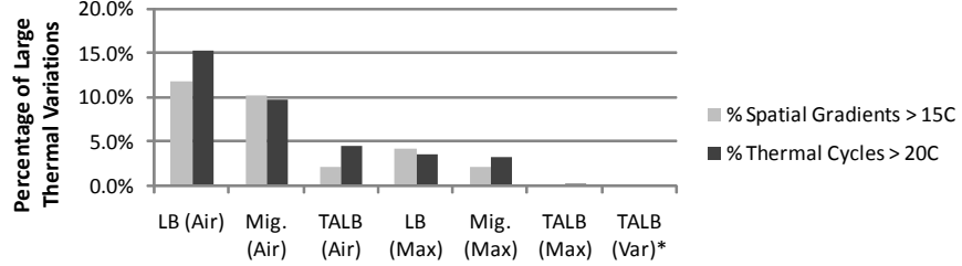
Fig. 10. Thermal variations (with DPM). (*) denotes our novel policy.
