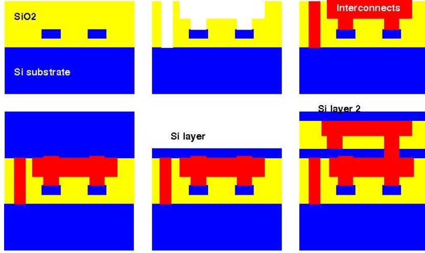
Fig. 3. MLBS process. [32]
