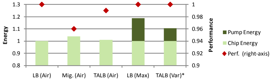
Fig. 11. Performance and Energy. (*) denotes our novel policy.
